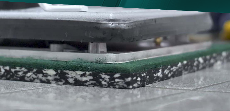
EXCENTER METHOD
